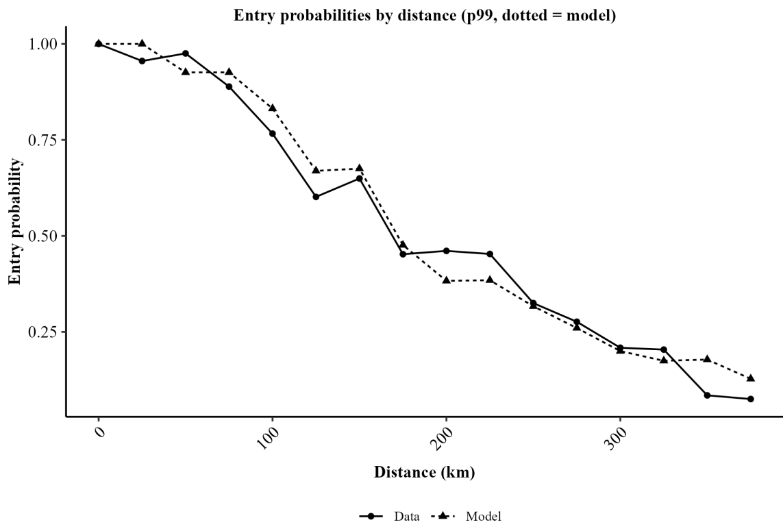
Figure 31: Extensive margin - 99th percentile
